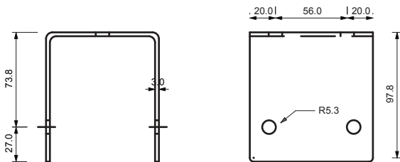
Hang bracket L type
